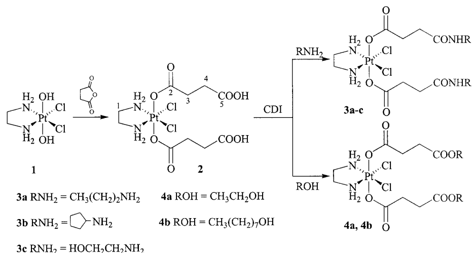
Figure 2. Synthesis of novel bis(carboxylato)platinum(IV) complexes and NMR numbering scheme.
