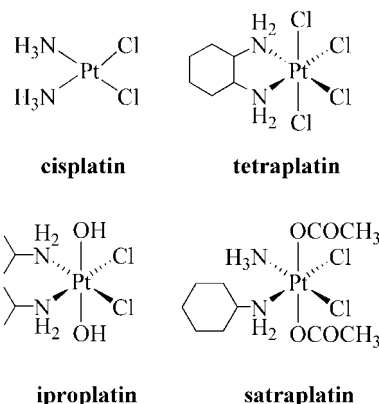
Figure 1. Chemical structures of the anticancer drug cisplatin and of tumor inhibiting platinum(IV) complexes in clinical evaluation. Tetraplatin and iproplatin were abandoned.
