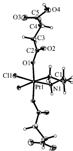
Figure 3. ORTEP diagram of 2 displaying thermal ellipsoids at 50% probability (the solvent molecule has been omitted). Selected bond lengths [Å] and angles [°]: Pt–N1 2.0541(10), Pt–Cl1 2.3175(5), Pt–O1 2.0113(12), O1–C2 1.3095(16), C2–O2 1.2235(16), C2–C3 1.5122(19), C3–C4 1.519(2), C4–C5 1.497(2), C5–O3 1.234(2), C5–O4 1.3070(18); O1–C2–O2 126.42(13), O3–C5–O4 123.13(15).
